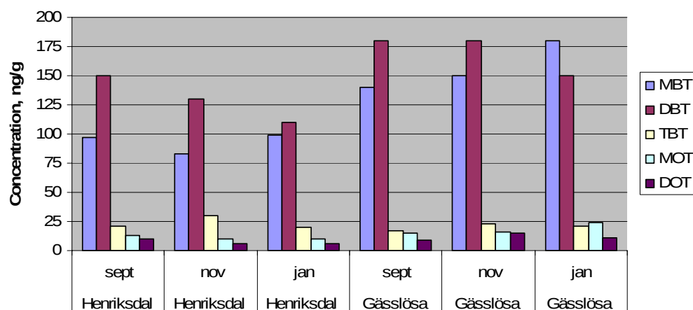
Figure 13. The temporal variation of organotin concentrations in sewage sludge at Henriksdal and Gässlösa sewage treatment plants.
